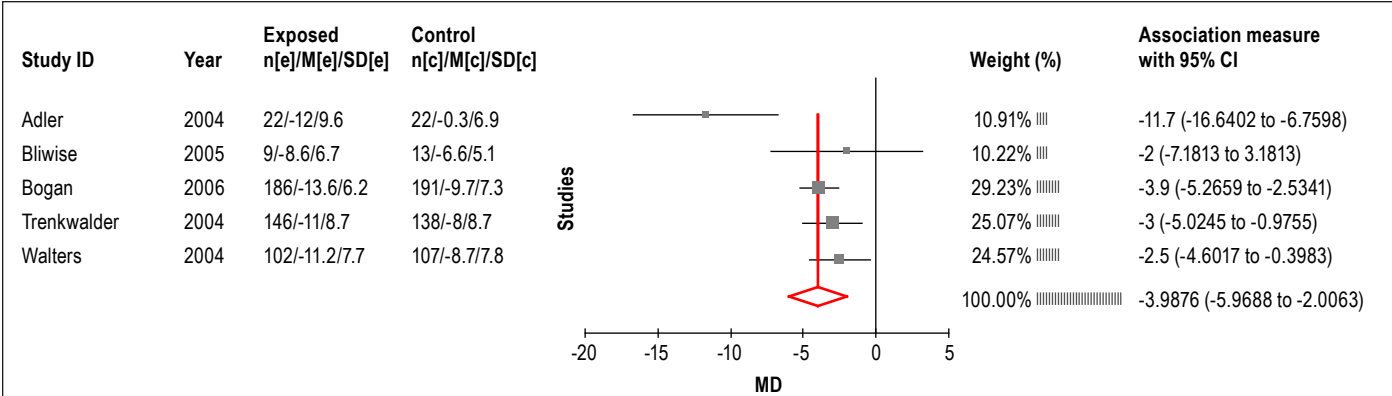
Figure 3—Meta-analysis of ropinirole IRLS data, improvement over placebo.
